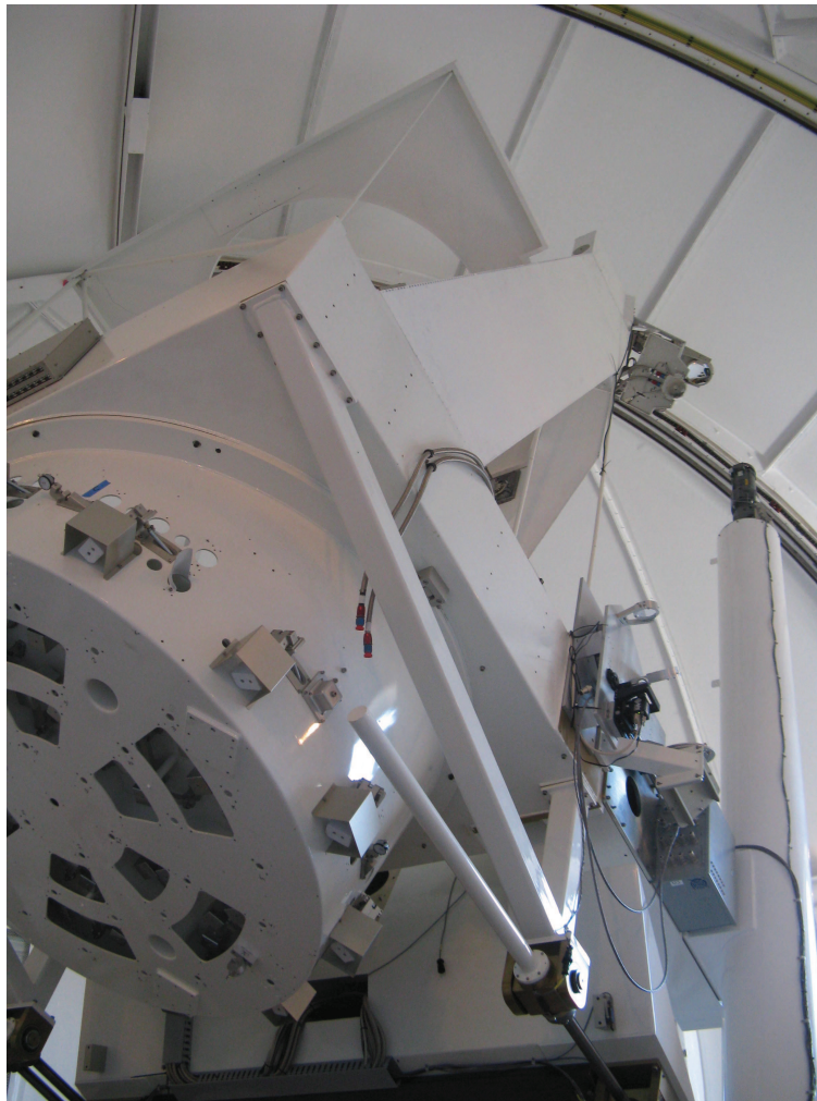
Figure 2: The NST mirror cell (lower left), secondary mirror on hexapod (upper middle), M3 complex with wavefront sensing system (lower right), one counterweight for right ascension balance (extreme right), and aperture shade (middle top).
