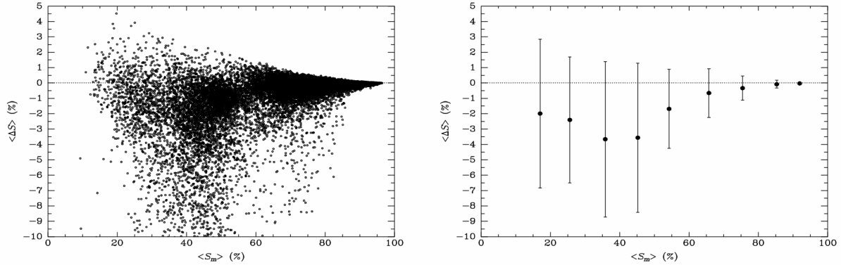
Fig. 7: Differences between Marechal-predicted and measured Strehl ratios for the individual frames (left) and in 10% bins.
