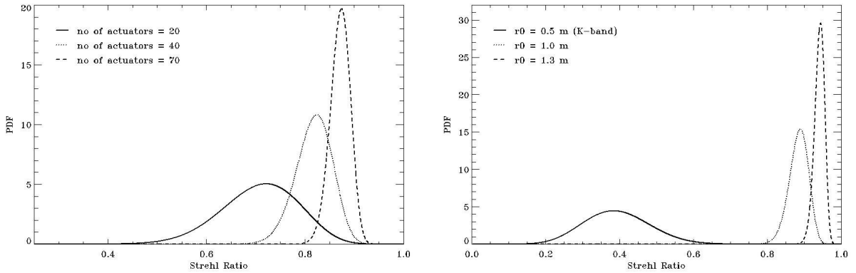
Fig. 11: (Left) Distributions of the Strehl ratio for three levels of actuator density, r_0 = 0.8\text{m} (K-band) and (Right) for three levels of turbulence strength when number of actuators is constant.
