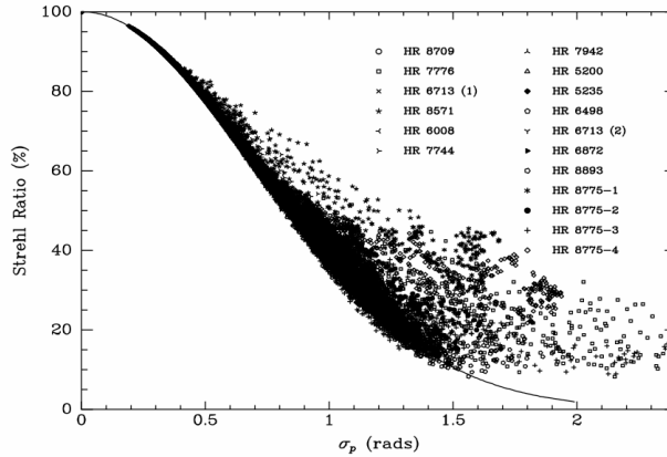
Fig. 5: The Marechal approximation (solid line) compared to the measurements of S and \sigma_p from the AEOS data.
