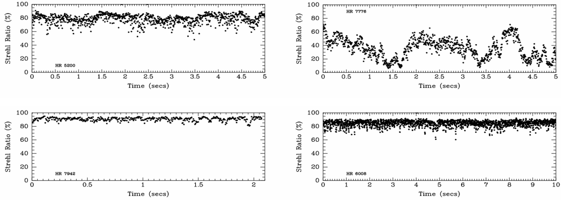
Fig. 3: Instantaneous Strehl ratio measurements from AEOS.
