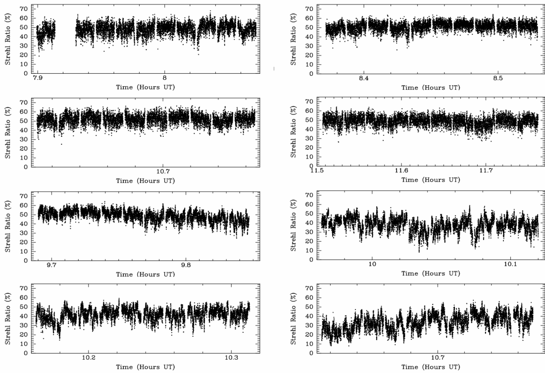
Fig. 1: Instantaneous Strehl ratio measurements from Lick Observatory.
