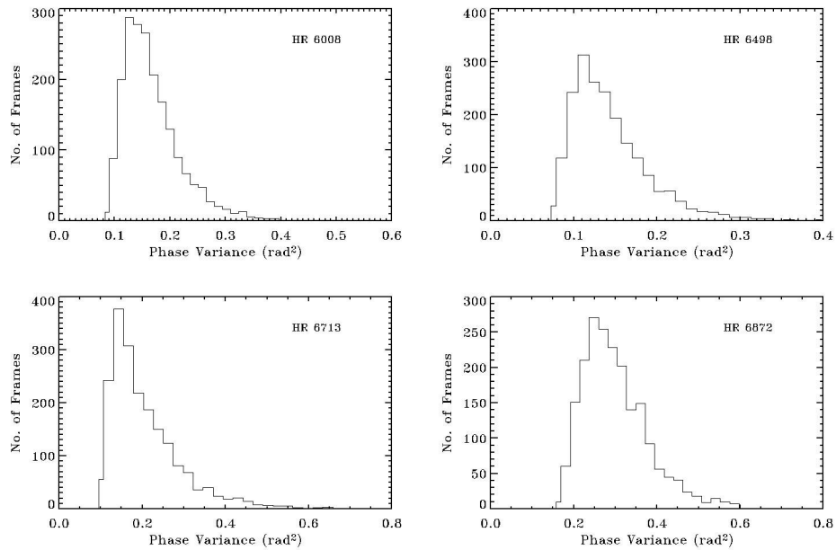
Fig. 8: Histograms of the phase variance for stars HR 6008, HR 6498, HR 6713 and HR 6872.
