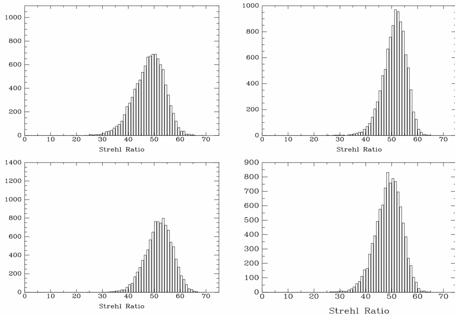
Fig. 2: Distribution of Strehl ratios for the top four plots in Figure 1. Note the similar non-Gaussian behavior with negative skewness.
