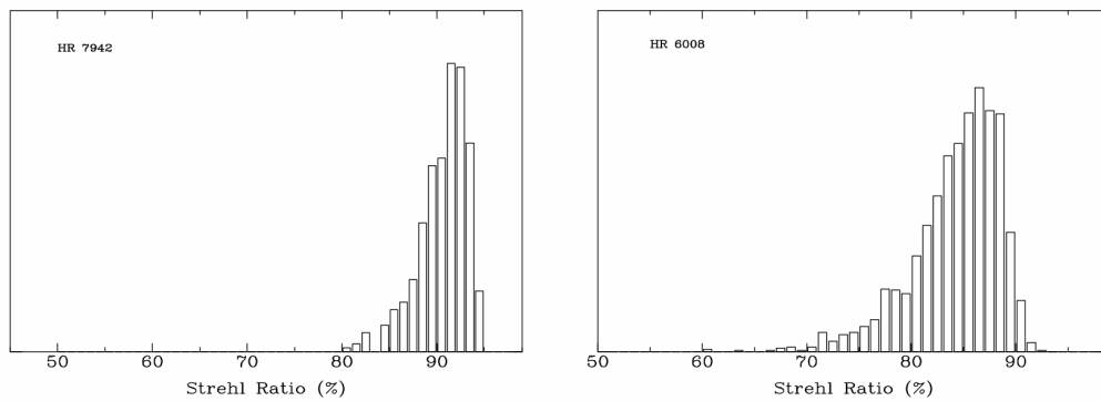
Fig. 4: Distribution of Strehl ratios for the bottom plots in Figure 3. Note the similar non-Gaussian behavior with negative skewness.
