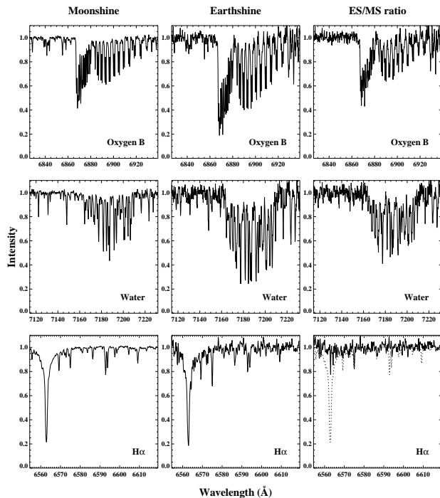
Fig. 5. — The spectrum of the moonshine, earthshine and the ratio of the two in the spectral regions of Oxygen A (top row), water (middle row) and H\alpha (bottom row).
