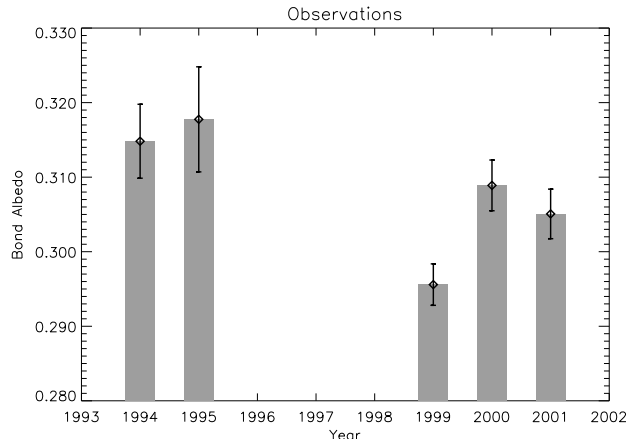
Fig. 3. — The earth's mean annual Bond albedo for each year in our observational earthshine record. The number of nights included in each year are tabulated in Table 1. Error bars represent \pm 1\sigma deviation from the mean.
