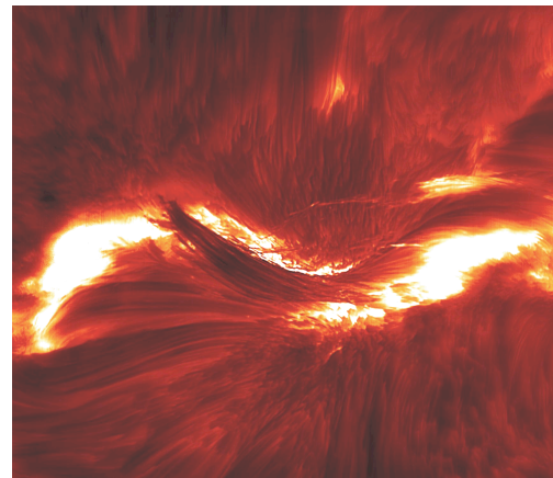
Figure 1: Flare seen in chromosphere in H\alpha center-line. The image is for NOAA Active Region 11817 on 11 August 2013 and the FOV of 50'' \times 50'' is spanned by the C2.1 flare’s impulsive phase. Post-flare loops can be seen running right-left covering parts of the right-left flare emissions.
