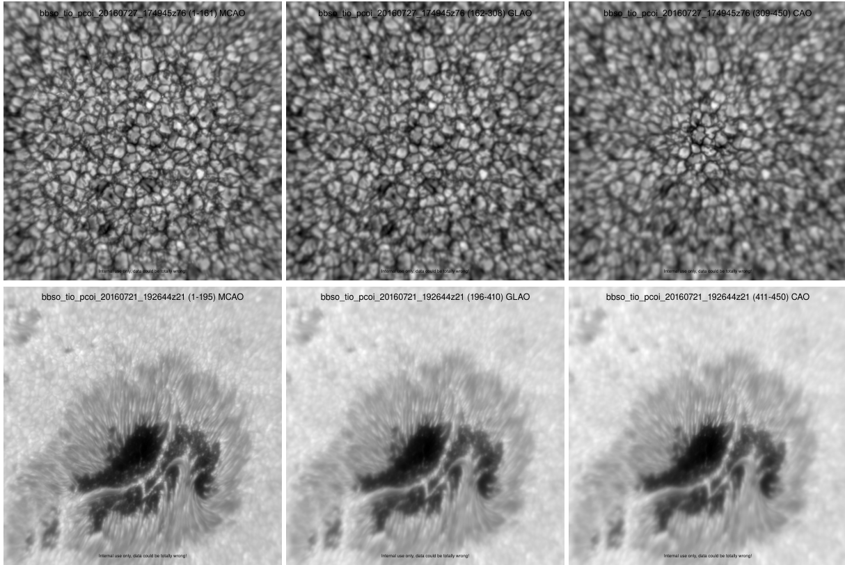
Figure 2: The Sun observed in a field of view of 53'' \times 53'' with MCAO, GLAO, and CAO correction with Clear on the NST through a filter for the titanium oxide line ( 705.7 \pm 5 nm). The top row shows a quiet region of the Sun between 10:49:45 and 10:50:16 local time on July 27th, 2016. The bottom row shows a sunspot in active region NOAA 12567 on July 21st between 12:26:44 and 12:27:24. Each image shows the sum of the images within a block with MCAO (left), GLAO (middle), and CAO (right) correction in a continuous burst of 450 frames recorded. No image reconstruction or contrast enhancing methods were applied. Real-time movies are available online ( GIVE ONLINE LOCATIONS??? ).
