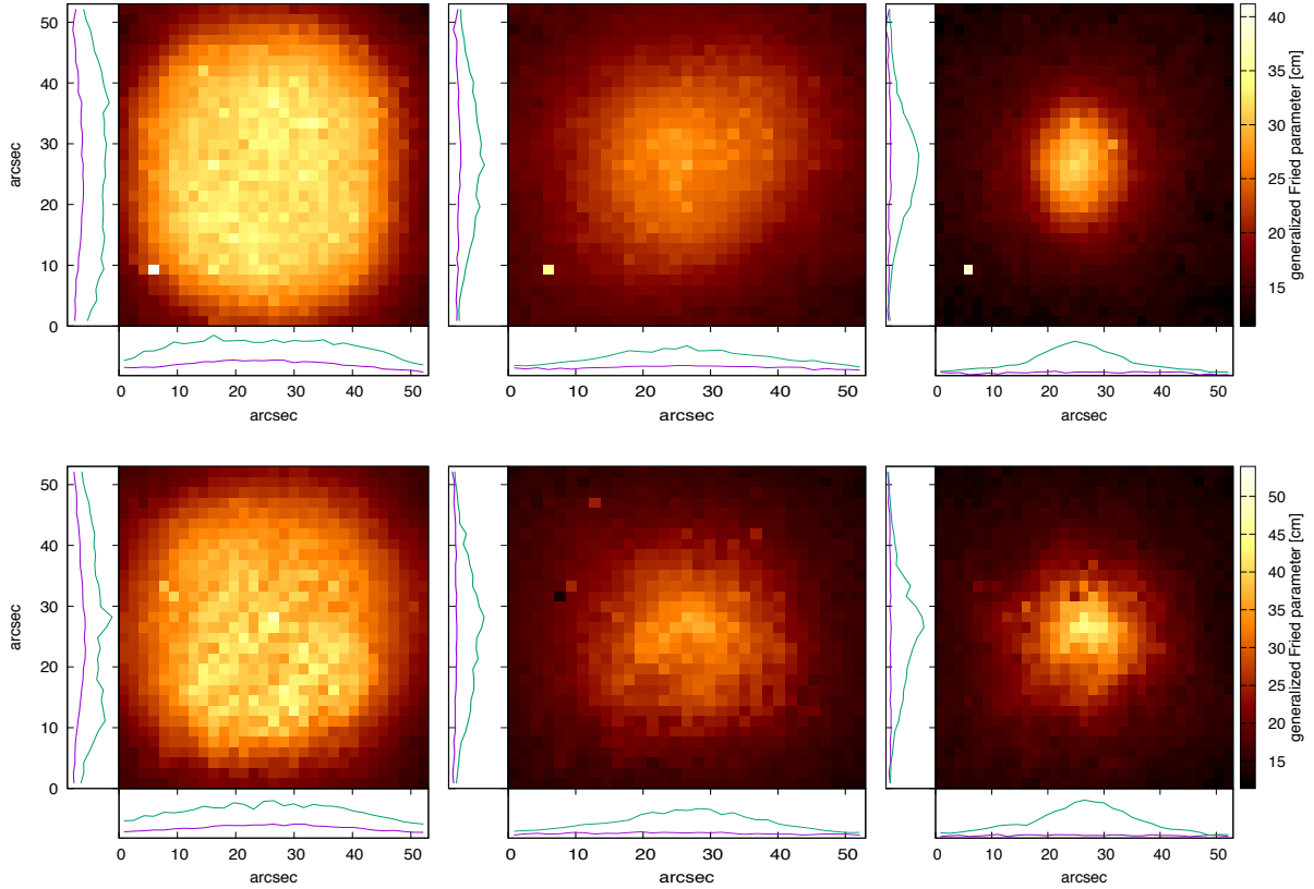
Figure 3: Generalized Fried parameter (?) across the field of view in the images shown in Fig. 1. The green lines along the ordinate and abscissa represent the relative intensities down and across the middle of the field, whereas the purple lines represent the corresponding relative intensities along the margins. For both rows, the full-width at half-maximum in the CAO green is \sim 10'' , while that for the MCAO is \sim 30'' .
