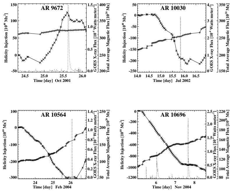
Figure 6: Time profiles of helicity injection, magnetic flux and GOES X-ray flux for 4 active regions. The helicity is shown as crosses; the dotted lines are the GOES X-ray flux and total average magnetic flux are shown as diamonds. The flux is averaged of the absolute sum of positive and negative fluxes.
