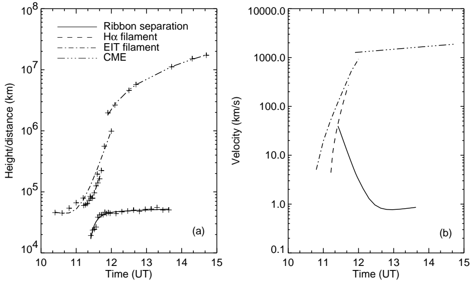
Figure 5: Left panel: time profiles of the flare ribbon separation, filament heights measured from KSO and EIT images of September 12, 2000, and CME heights measured by Dr. Yashiro ( http://cdaw.gsfc.nasa.gov/CME_list/ ). The lines indicate the least-squares fits to hyperbolic functions. Right: velocity profiles of the ribbon separation, filament, and CME derived from the fits of the height profiles.
