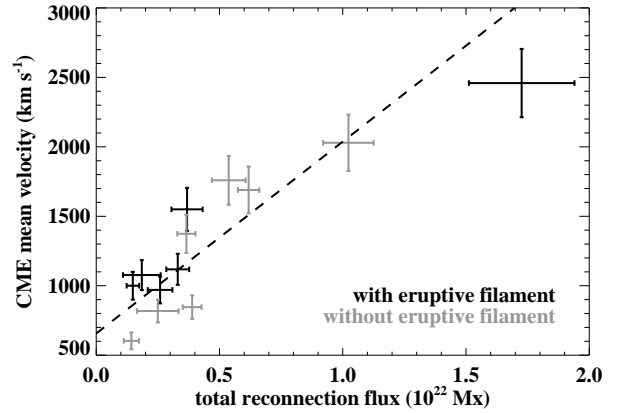
Figure 9: Scatter plot of CME velocities vs. total reconnection flux for 13 events. Dark and gray colors indicate events associated with erupting and non-erupting filaments, respectively. The dashed guide-line shows the least-squares linear fit to the data points (Qiu and Yurchyshyn, 2005).
