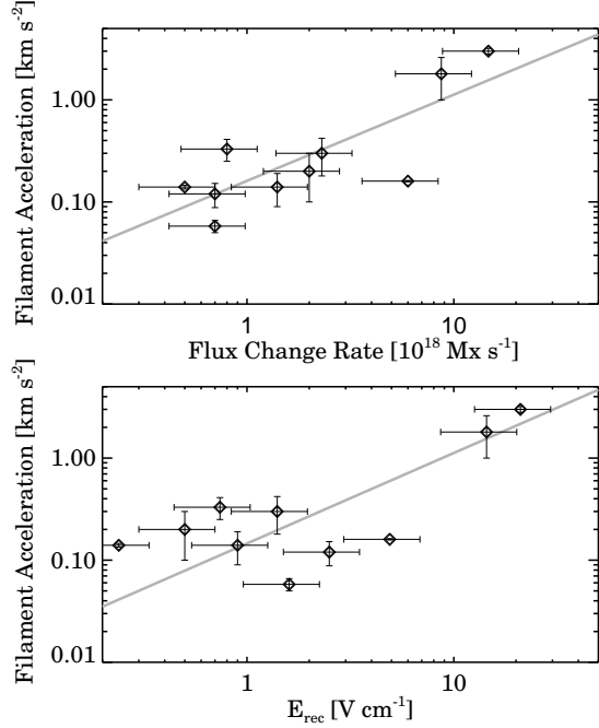
Figure 8: Top: Scatter plot of maximum filament acceleration vs. maximum \Phi_{rec} ; Bottom: Scatter plot of maximum filament acceleration vs. maximum E_{rec} . Error bars attached to each sign indicate the uncertainty of the measurement (Jing et al., 2005).
