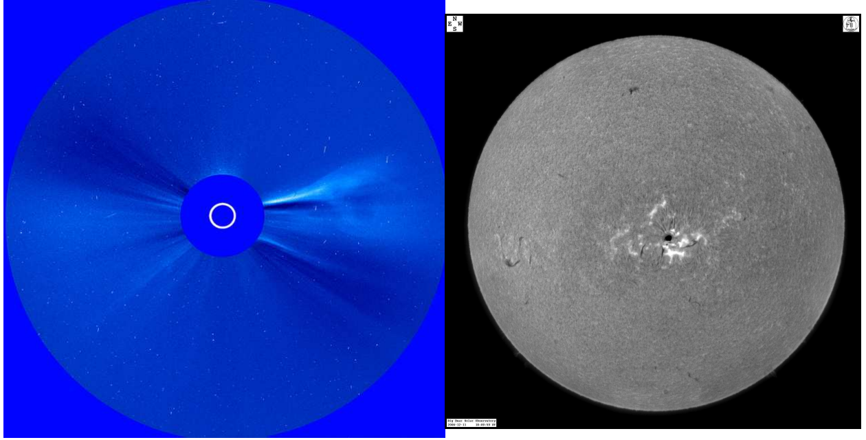
Figure 4: Comparison of a CME observed on December 9, 2006 as observed by COR2/SECCHI on board STEREO (left) and a full disk Halpha obtained at BBSO on December 11, 2006. This simulates the situation when the STEREO has a view angle of about 60 degrees away from earth's observations. Then the center region active region's CME will be view clearly as limb event.
