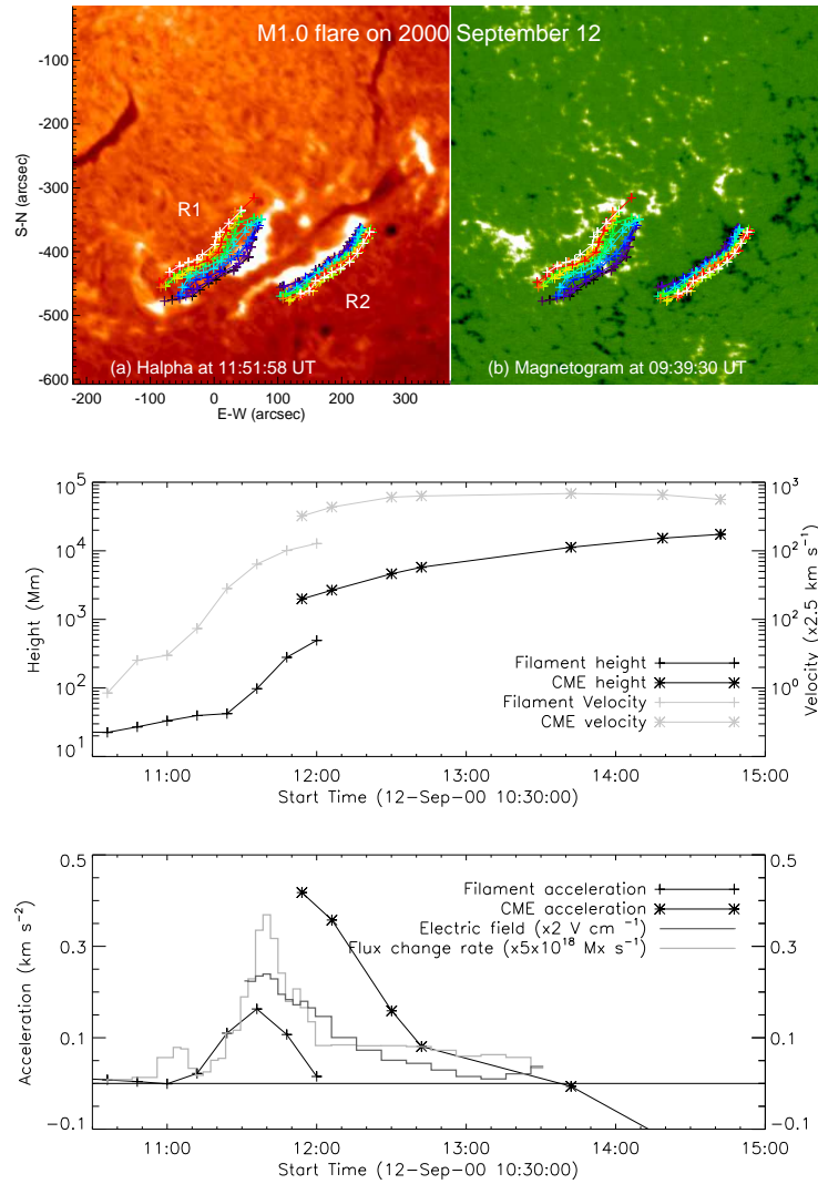
Figure 7: Evolution of flare, filament, and CME in the 2000 September 12 event. Top panels: snapshot of an M1.0 flare in H \alpha observed by KSO on 2000 September 12 and corresponding MDI magnetogram. Plus signs are trajectories of the ribbon fronts; colors from purple to white indicates a 2 hr time lapse from 11:00 to 13:00 UT. Middle panel: measured heights and deduced velocities of the filament and CME. Bottom panel: deduced acceleration of the filament and CME, compared with E_{rec} and \phi_{rec} (Qiu et al., 2004).
