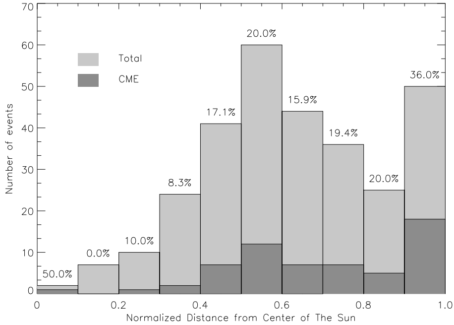
Figure 1: Distribution of filament disappearance as function of the distance from the disk center. The lighter histogram is the total number of events, and the darker histogram is the number of events with associated CMEs found from the LASCO data. We also indicated at the top of each bar the percentage of events for which LASCO events have been identified.
