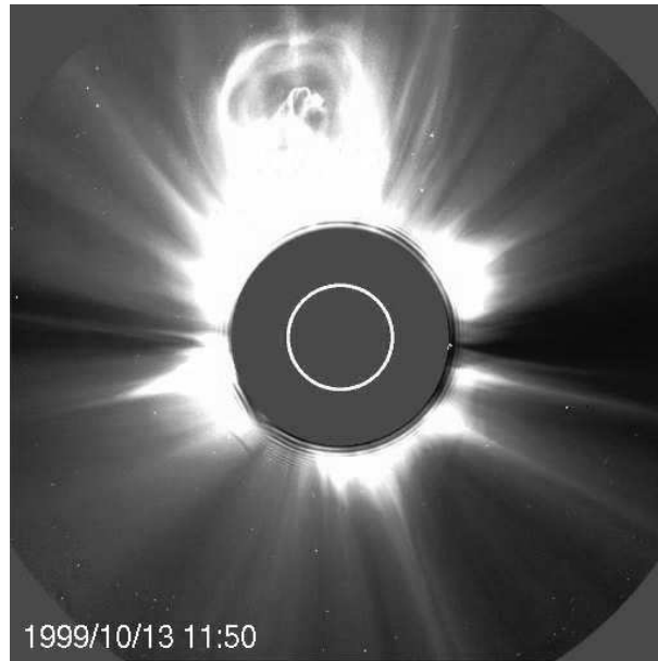
Figure 3: The LASCO C2 image shows the CME corresponding to the filament disappearance in Figure 2.
