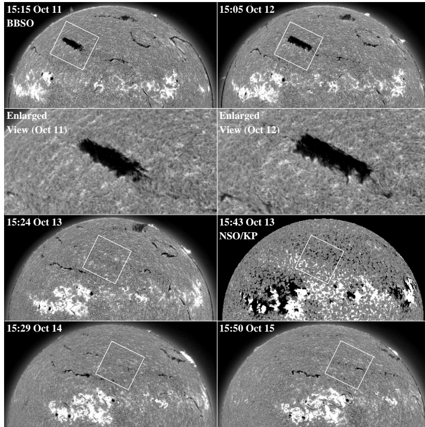
Figure 2: The sequence of H\alpha full-disk images demonstrating the disappearance of a major filament inside the white box. A Kitt Peak magnetogram at 15:43 on October 13 is also included to show the magnetic configuration. In the second row, we show a magnified field of view from the same images in the first row to demonstrate that the fine structure can be resolved by our full disk images.
