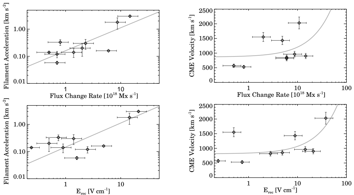
Figure 8: Top-left: Scatter plot of maximum filament acceleration vs. maximum \phi_{rec} ; Bottom-left: Scatter plot of maximum filament acceleration vs. maximum E_{rec} . Top-right: Scatter plot of CME velocity at C2 vs. maximum \phi_{rec} ; Bottom-right: Scatter plot of CME velocity vs. maximum E_{rec} . Error bars attached to each sign indicate the uncertainty of the measurement (Jing et al., 2005).
