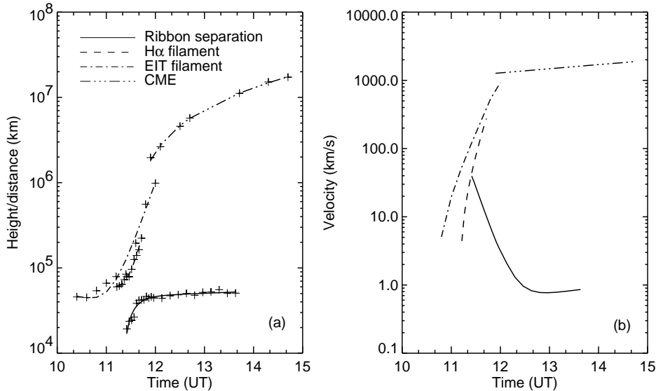
Figure 5: Left panel: time profiles of the flare ribbon separation, filament heights measured from KSO and EIT images, and CME heights measured by Dr. Yashiro ( http://cdaw.gsfc.nasa.gov/CME_list/ ). The lines indicate the least-squares fits to hyperbolic functions. Right: velocity profiles of the ribbon separation, filament, and CME derived from the fits of the height profiles.
