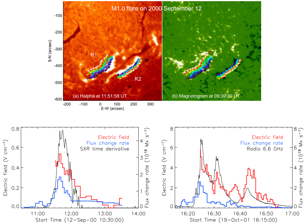
Figure 7: Top panels: snapshot of an M1.0 flare in H\alpha observed by KSO on 2000 September 12 and corresponding MDI magnetogram. Plus signs are trajectories of the ribbon fronts; colors from purple to white indicates a 2 hr time lapse from 11:00 to 13:00 UT. Bottom panels: Left: magnetic reconnection rate in terms of E_c (red) and \phi_c (blue) in comparison with the time derivative of the GOES soft X-ray emission (dark) for the M1.0 event on 2000 September 12. Right: magnetic reconnection rate in terms of E_c (red) and \phi_c (blue) in comparison with the microwave light curve at 6.6 GHz (dark) for the X1.6 event on 2001 October 19 (Qiu et al., 2004).
