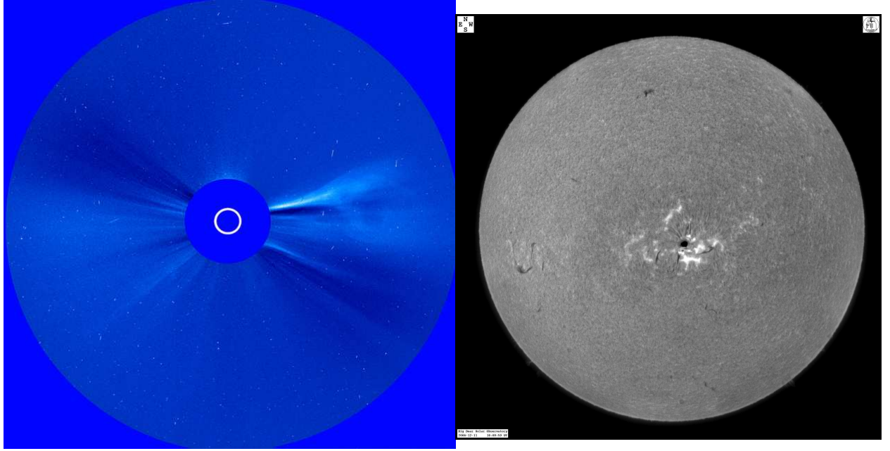
Figure 4: Comparison of a CME observed on December 9, 2006 as observed by COR2/SECCHI on board STEREO (left) and a full disk Halpalpha obtained at BBSO on December 11, 2006. This simulates the situation when the STEREO has a view angle of about 60 degrees away from earth's observations. Then the center region active region's CME will be view clearly as limb event.
