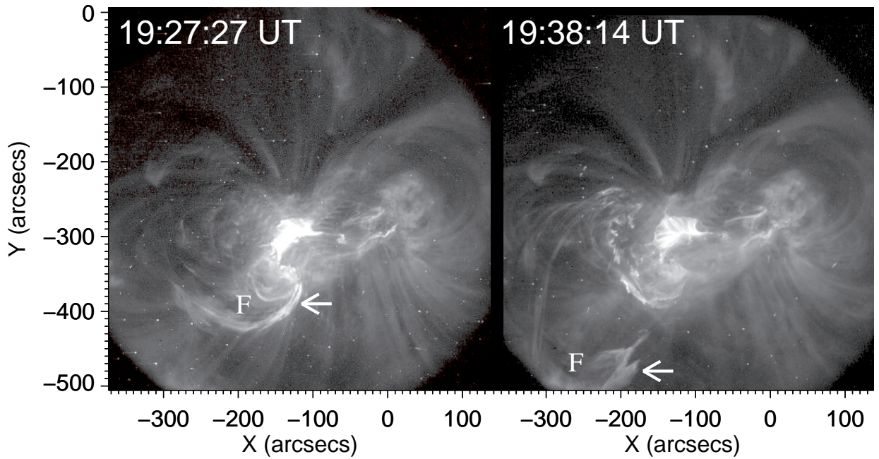
Fig. 3.— TRACE 195 Å images showing the brightening of a large loop (denoted by arrow) that is co-spatial with the filament (“F”), and their final eruption after \sim 19:35 UT.
