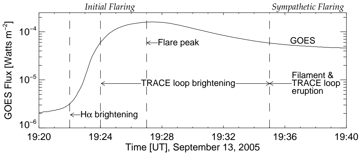
Fig. 4.— Time line of the 2005 September 13 X1.5 event described on the light curve of GOES soft X-ray flux at the 1–8 Å channel, showing the starting time of H \alpha brightening ( \sim 19:22 UT), TRACE loop brightening interval ( \sim 19:24 – 19:35 UT), the flare peak time in GOES ( \sim 19:27 UT), and the time of filament and TRACE loop eruption ( \sim 19:35 UT). See § 3 for detailed discussion.
