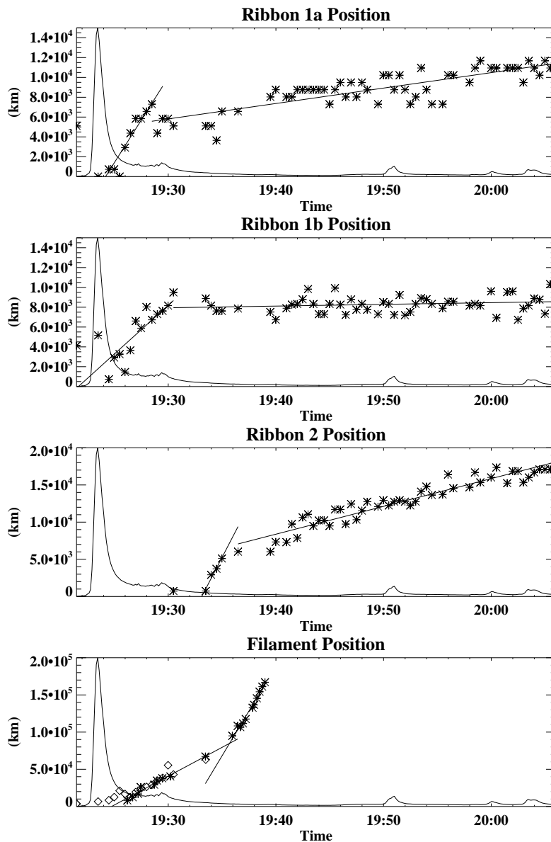
Fig. 2.— The position of front of the three moving flare ribbons as a function of time. The solid line is the light curve of microwave at 10 GHz observed by OVSA. The bottom panel shows the filament heights. Diamonds are points based on BBSO H\alpha observations, while the stars are based on TRACE 195 Å observations. Straight lines are fittings to derive speeds of motions.
